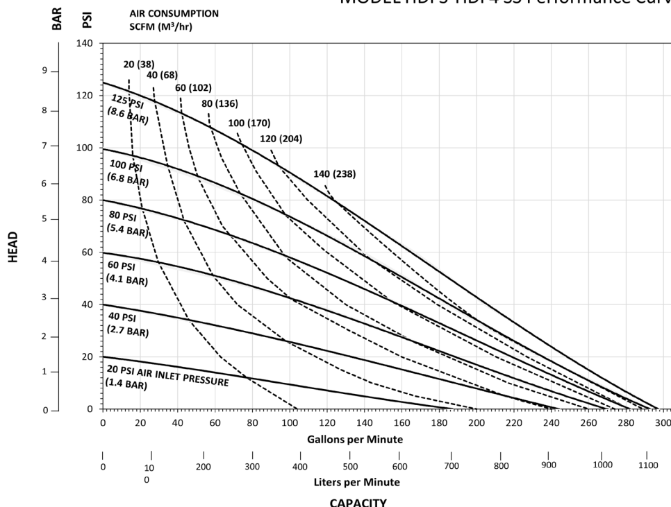
MODEL HDF3-HDF4 SS Performance Curve
