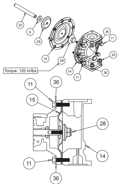
Diaphragm Orientation Intall diaphragm as shown above.
