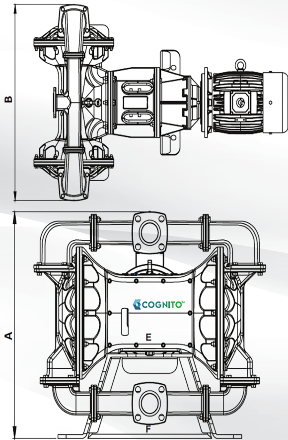
Dimensions & Weight - Inline
